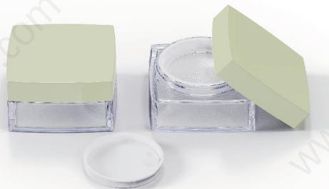
C147C1 | Size:L68.78*W68.78*H37.85mm Capacity:85.8ml/OFC 65.6ml/Filling Line Material:SAN(Cap) +PP(Inner Cap) +PP(Disc)+PP(Siexe)+PP(Gauze Holde) +SAN(Jar)+SAN(Bottom)+Liner
